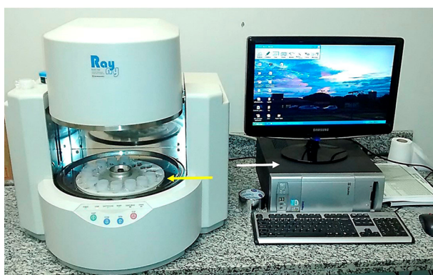
Figure 8. Equipment for the non-destructive biochemical analysis by energy dispersion EDX-720 (EDXS – X-ray fluorescence)
